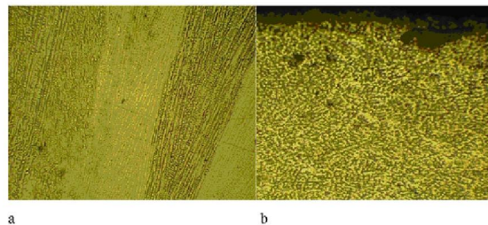
Fig. 3. Microstructure of austenite metal of welded joint of DN300 pipeline (steel type is 08X18H10T according to Russian standard designation), which was obtained: a – without ultrasonic effect, b – with ultrasonic effect (×125 magnification).
