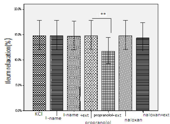
Figure 2: Comparison of the anti-contraction effect of Kelussia hydroalcoholic extract concentration (20%) on contraction caused by potassium chloride (60mM), in the presence and absence of L-NAME (1μM, 30 min, n=8), propranolol (1μM, 30 min, n=8) and naloxone (1μM, 30 min, n=8).
