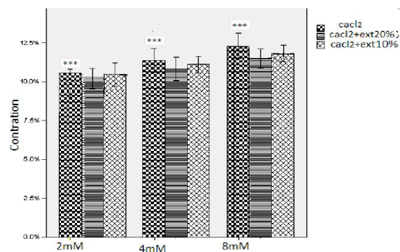
Figure 3: Comparison of calcium chloride cumulative concentrations (2, 4, 8 mM) on ileum in free calcium tyrode solution with high concentration of potassium chloride (60mM) in the absence of extract followed by incubating tissue in cumulative concentration of extract (10% and 20%) for 3 minutes.
