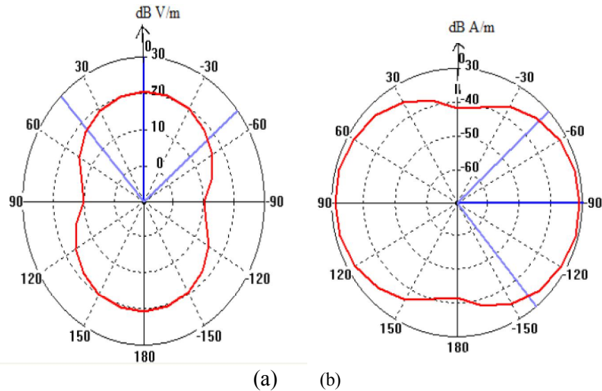
Fig.5. Radiation Patterns of the proposed MIMO antenna system (a) E Plane (b) H Plane
