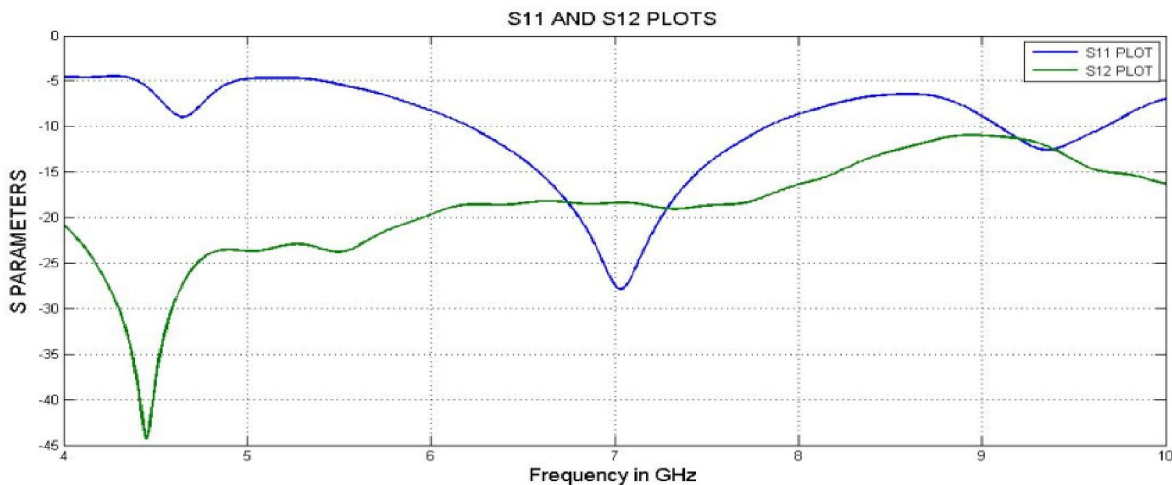
Fig 2. S-Parameters of the proposed Knee shaped patch antenna
