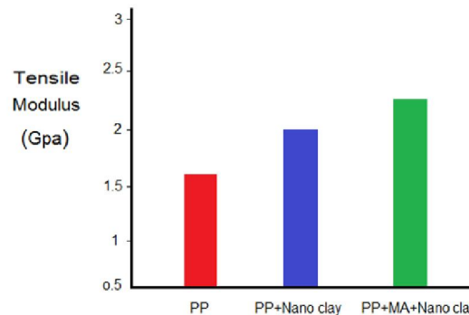
*Fig (8)-tensile modulus in different states
