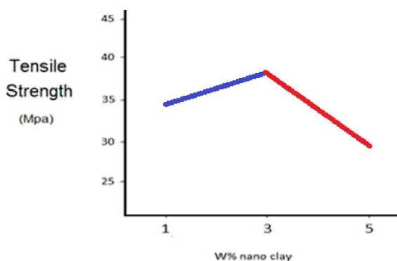
*Fig (7): tensile strength of the Nano composite with different percentages of modified Nano clay.
