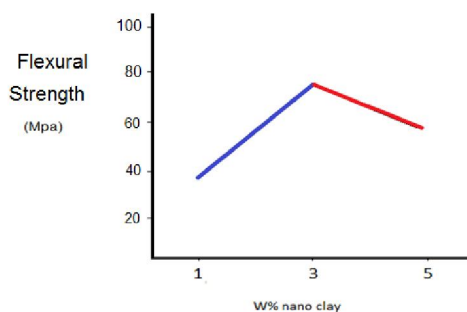
Fig (5): bending strength of a Nano composite with different percentages of the modified Nano clay.
