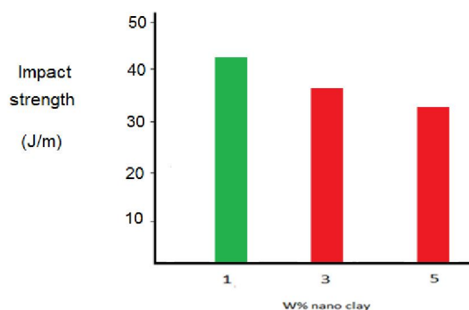
*Fig (9): Shock strength of the Nano composite with different modified Nano clay.
