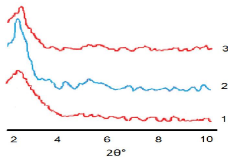
*Fig (3)-modified Nano clay 3 (5%); 2(3%); 1(1%) in Nano composite
