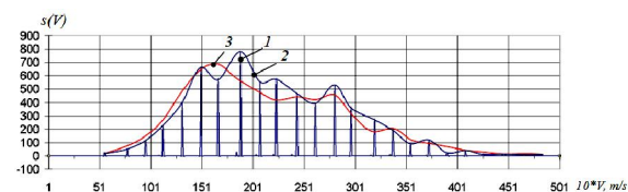
Fig.2. Graph (1) according to the number of a wind impulses in Anchorage on wind speed ( m/s ) in the period from 01.01.1973 on 31.08.1987 (resolution dV=0.1 m/s ):
