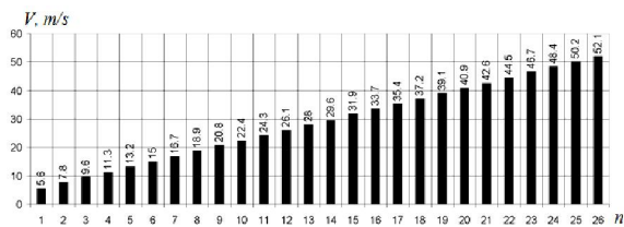
Fig.4. The diagram of dependence of the wind formation speed from conventional peak non V(n) their statistical distribution in Anchorage
