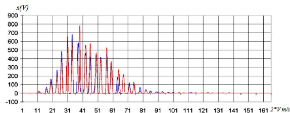
Fig.1. The graph of the wind impulses amount in Anchorage on wind speed (resolution dV=0.5 m/s ):
