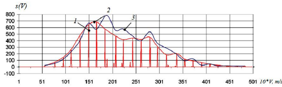
Fig 3. Graph (1) according to the number of a wind impulses in Anchorage on wind speed (m/s) in the period from 01.01.1995 on 31.08.2009 (resolution dV=0.1 m/s):
