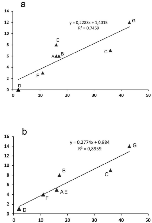
Figure 4. Linear correlation between number of species and number of litophytes (a) and between number of species and number of xerotherms (b). A, B, C...G – signature of climbing route
