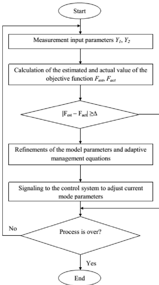
Figure 2. Proposed algorithm for adaptive management .
