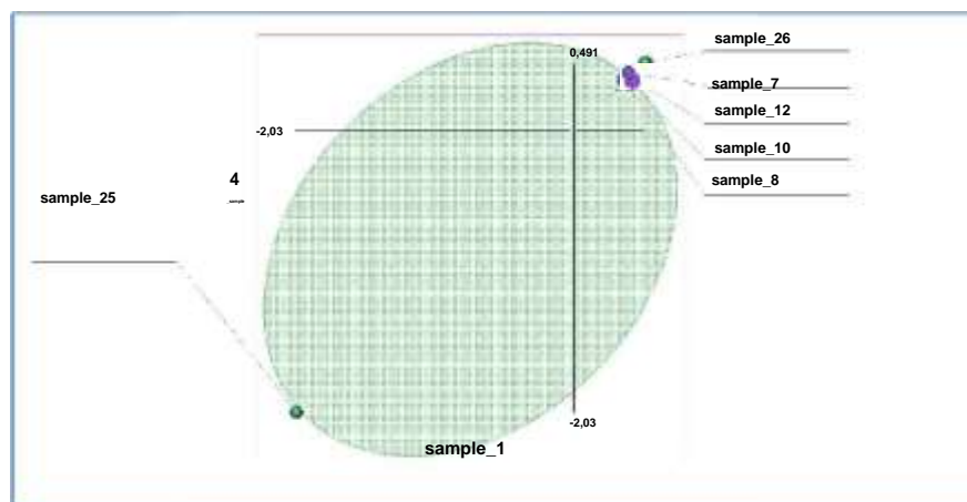
Fig. (9): PCA for the comparison between treated and un-treated samples with proline
