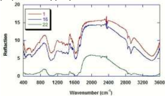
Fig. (6): Mid-infrared spectra for Jojoba under irrigation with quality of water (normal and saline water with 2500ppm and 5000 ppm) with 200 proline
