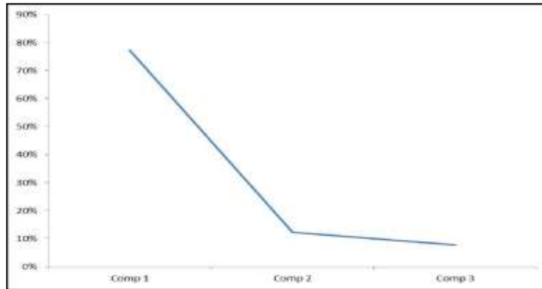
Fig. (8) Principle component analysis
