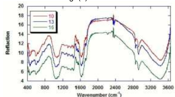
Fig. (4): Mid-infrared spectra for Jojoba under irrigation with saline water (5000 ppm) with and without proline
