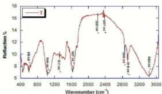
Fig. (1): Mid-infrared spectra for Jojoba under irrigation with tap water
