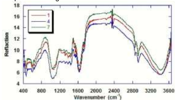
Fig.(3) Mid-infrared spectra for Jojoba leaves under fresh water
