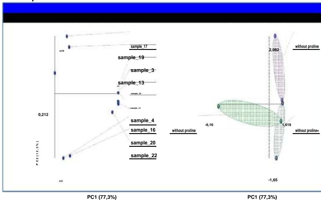
Fig. (7): PCA for the different treated plants
