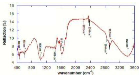
Fig. (2): Mid-infrared spectra for Jojoba under salt stress
