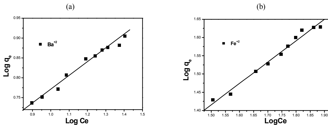
Figure 9: Freundlich Isotherm Plot for Adsorption of (a) Ba(II) and (b) Fe(II) by activated carbon (MA).
