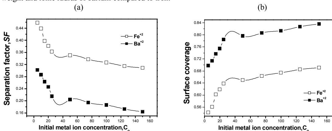
Figure 10: A plot of separation factor, SF and surface coverage, \theta against initial metal ion concentration of Ba(II) and Fe(II) for activated carbon adsorbent (MA).
