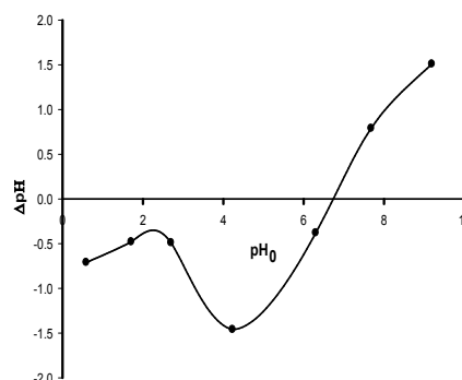
Figure 3. Point zero charge of activated carbon (MA).
