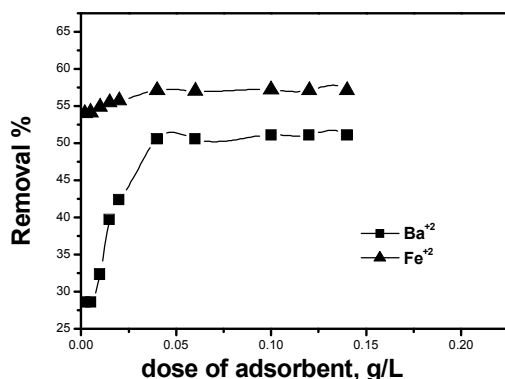
Figure 5: Effect of adsorbent dosage on adsorption of Ba(II) and Fe(II) by activated carbon(MA), initial concentration = 100 mg/L, contact time 30 min.
