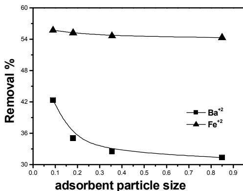
Figure 6: Effect of adsorbent particle size of adsorbent in the removal of Ba(II) and Fe(II) ions, initial concentration = 100 mg/L, 0.02 g/L adsorbent dose, contact time 30 min.
