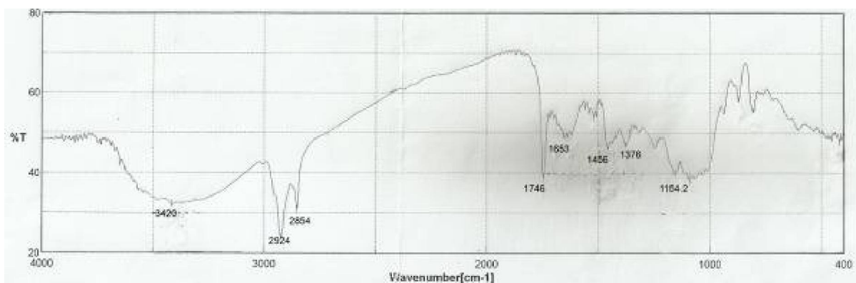
Figure 1. FT-IR Spectrum of activated carbon (MA).
