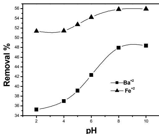
Figure 4: Effect of pH on adsorption of Ba(II) and Fe(II) by activated carbon(MA), initial concentration = 100 mg/L, 0.02 g/L adsorbent dose, contact time 30 min.
