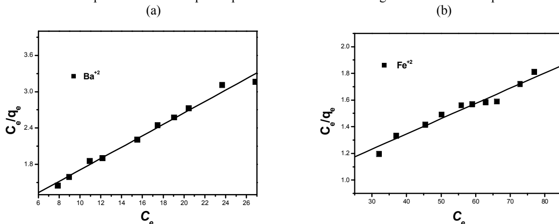
Figure 8: Langmuir Isotherm Plot for Adsorption of (a) Ba(II) and (b) Fe(II) by activated carbon (MA).
