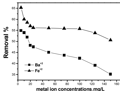
Figure 7: Effect of metal ion concentration on adsorption of Ba(II) and Fe(II) by activated carbon(MA), pH 7.5 \pm 0.5 , adsorbent dosage 0.02 g/L, contact time 30 min.
