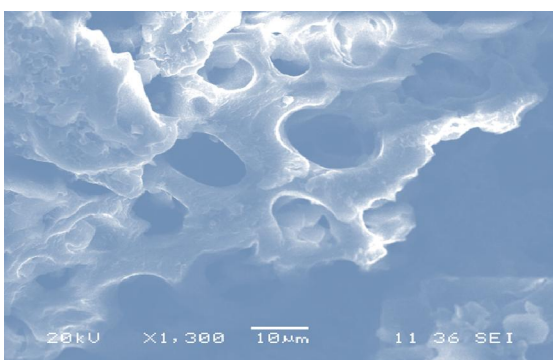
Figure 2. SEM photographs of the activated carbon (MA).
