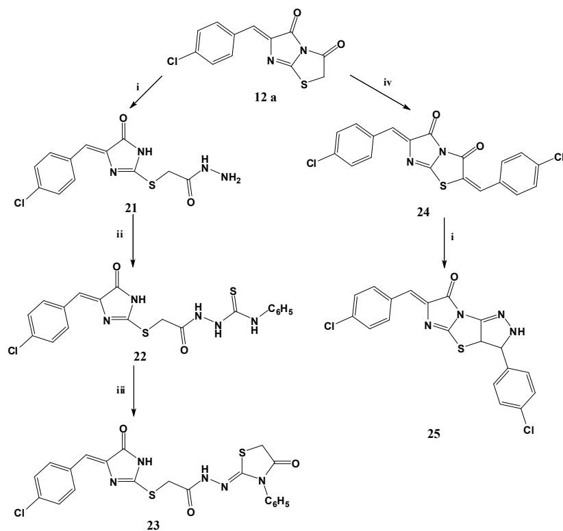
Scheme 5
