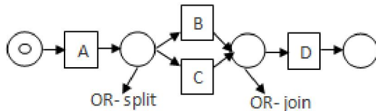
Figure 5: conditional routing
