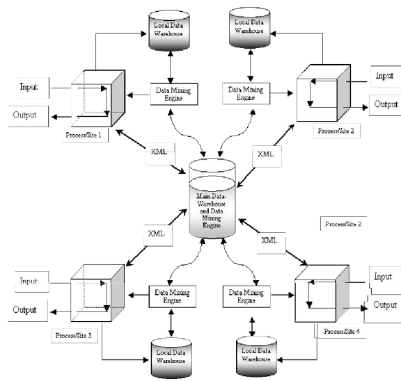
Figure 3. An Integrated Data Mining System Model
