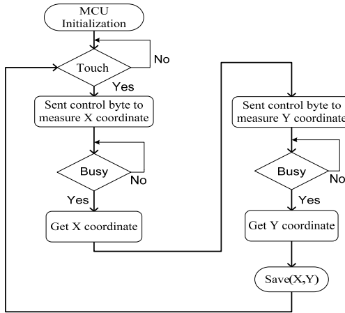
Figure 4. Flowchart of firmware design.
