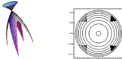
Figure 9: The image of singular S_{III_{23}} \equiv S_{III_{24}} and its contours
