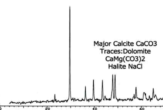
Fig. (6): XRD pattern of limestone sample
