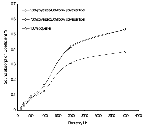
Fig.2, Effect of fiber type on fabric sound absorption at weight 400\text{g/m}^2
